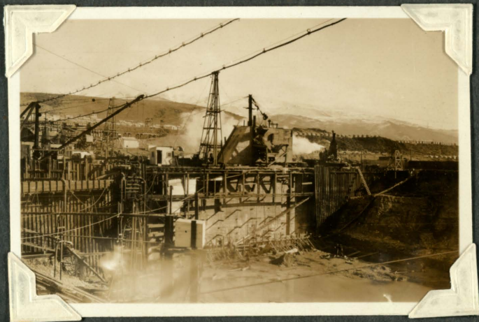
Cofferdam. Cut off wall excavation on right. Village houses in background. Drag-line excavator tipping into hopper.
