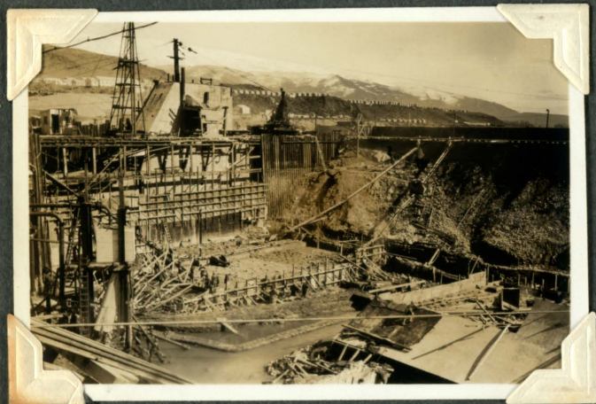
Midstream side of cofferdam Water approx. 40ft below river level outside. Leakage confined & directed by sandbags.
