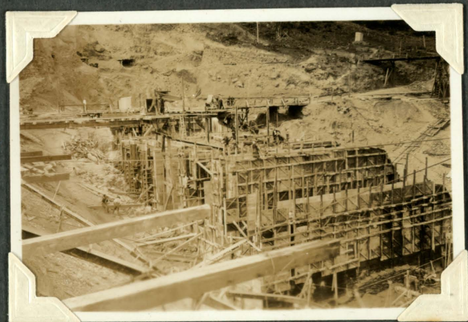
Upstream face of dam. Sluice gate frames being fitted in position.
