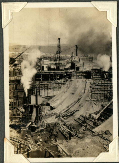
The closing section of dam almost completed.
