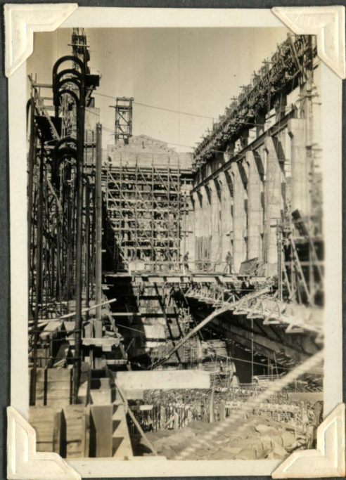
Crane runway in position on West wall of generator room.
