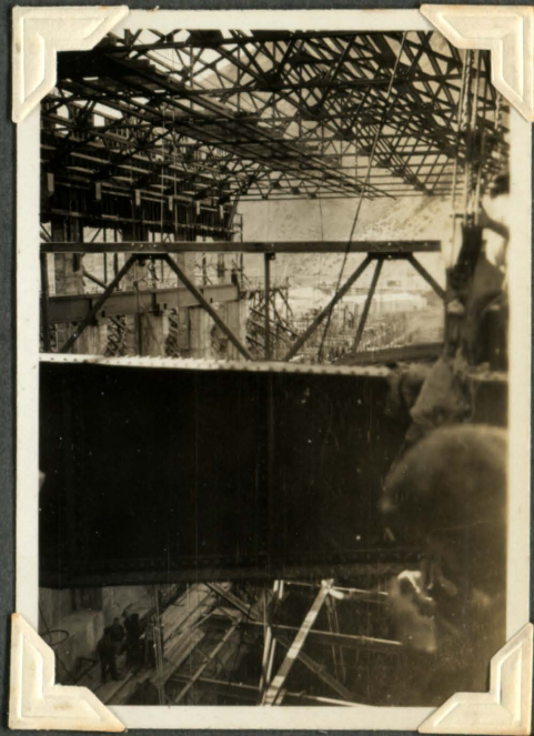
1 st Beam lifted to rail level. Auxillary beam attached to bogies in position.
