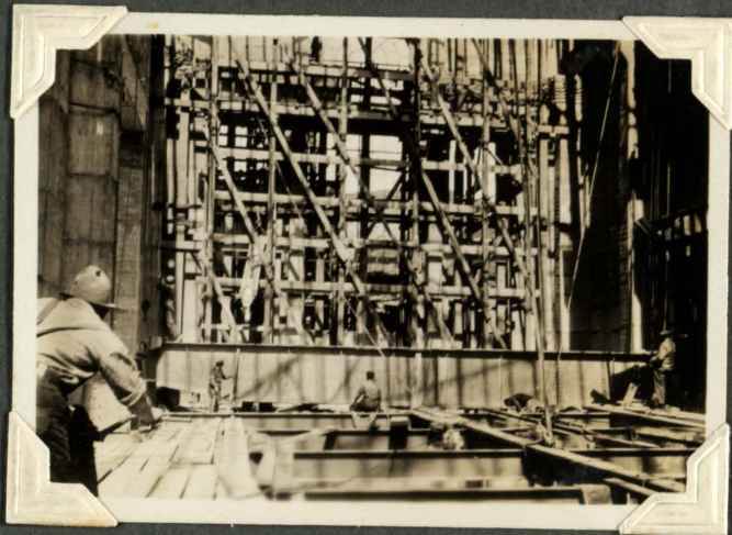
Lifting tackle being rigged Winch on left.
