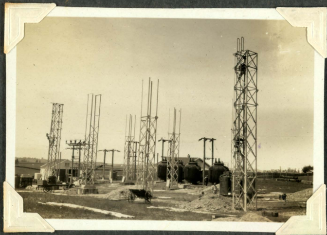
Self-cooled transfs. in background.
